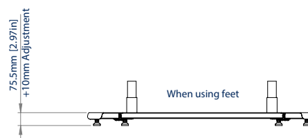
VISTA FRONTAL LEVELLING FEET
