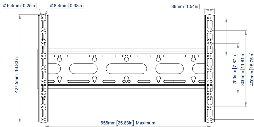
VISTA FRONTAL
