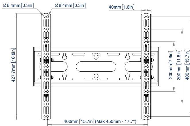
VISTA FRONTAL
