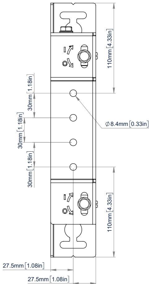
VISTA FRONTAL
