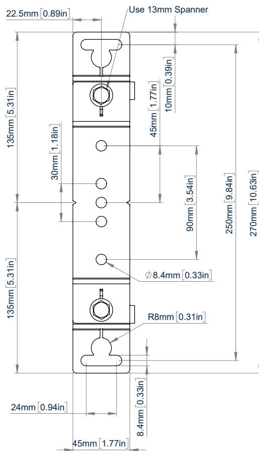
VISTA FRONTAL
