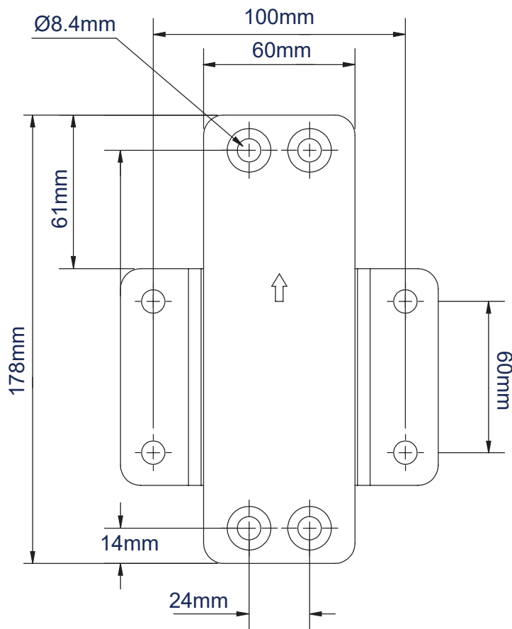
VISTA FRONTAL
