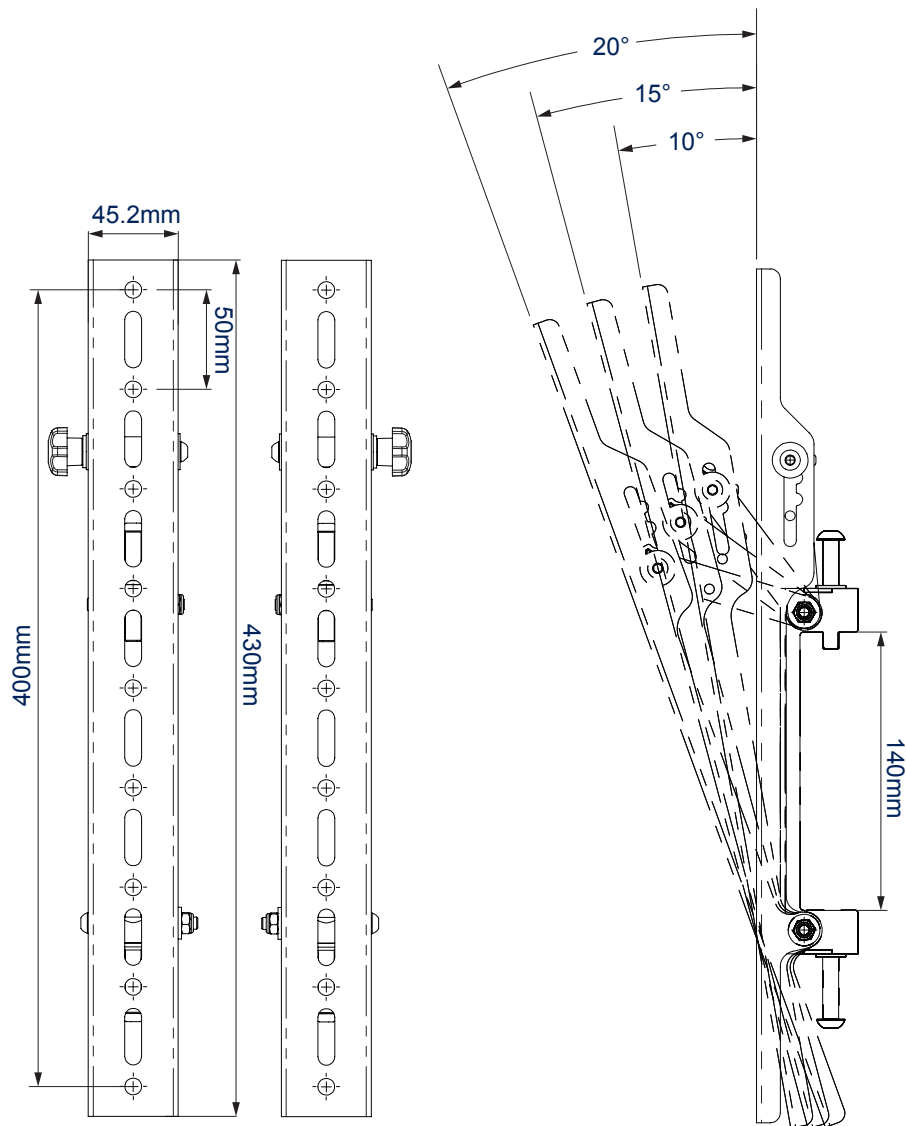
VISTA FRONTAL
