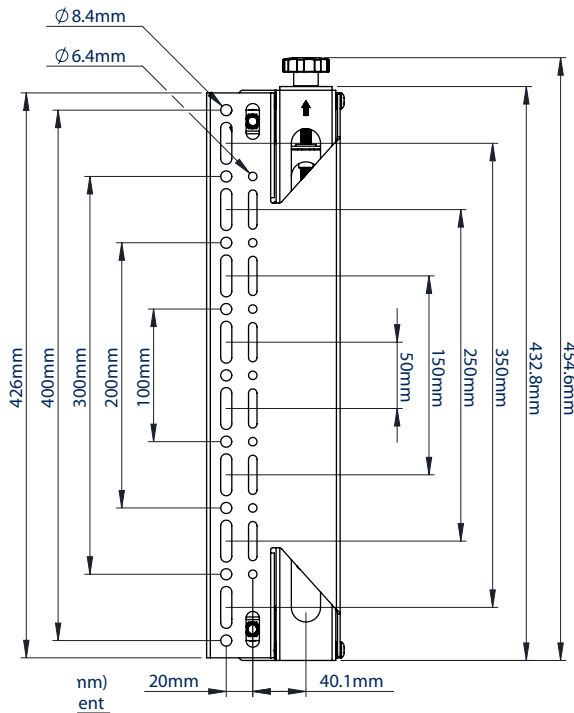
VISTA FRONTAL
