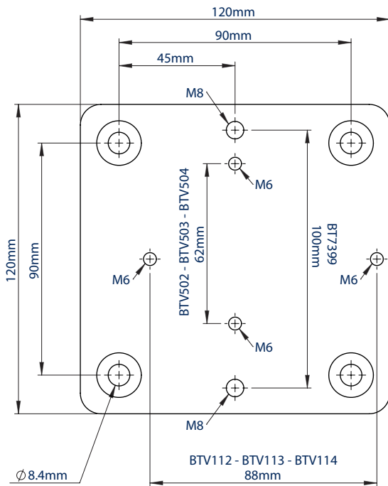
VISTA FRONTAL
