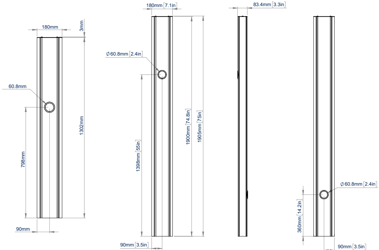
BT8385-130 VISTA FRONTAL
