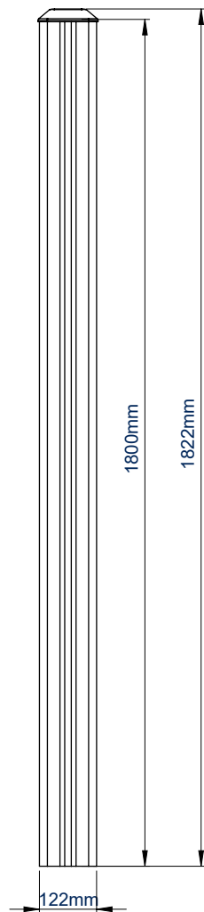
VISTA FRONTAL
