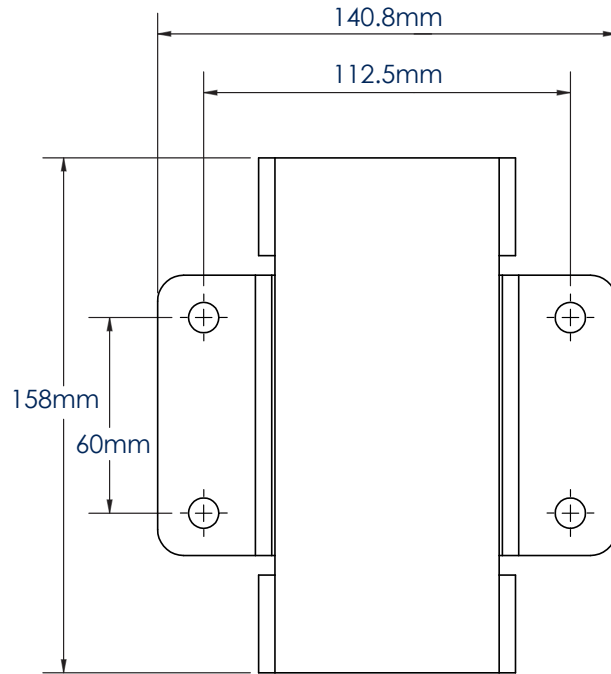
VISTA FRONTAL
