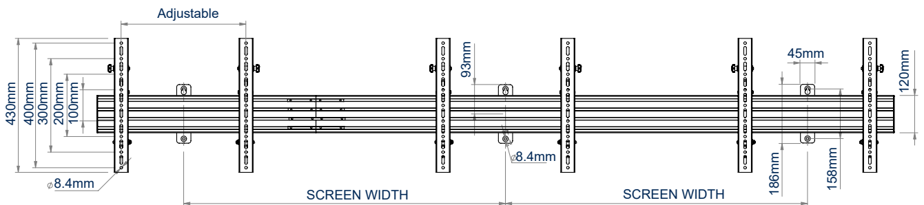
VISTA FRONTAL
