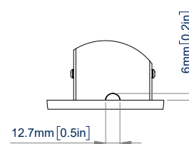
DETAIL A SCALE 1 : 3
