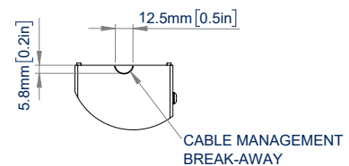
DETAIL A SCALE 1 : 3
