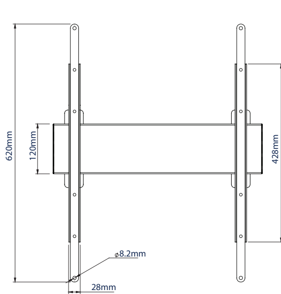
VISTA FRONTAL
