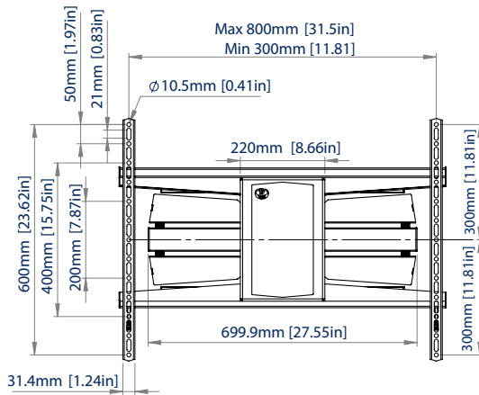
VISTA FRONTAL
