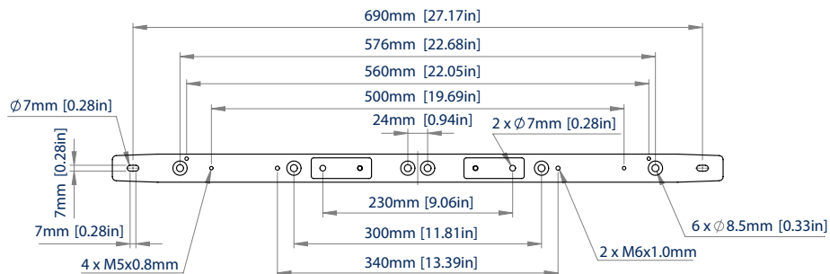
VISTA FRONTAL
