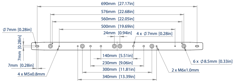
VISTA FRONTAL
