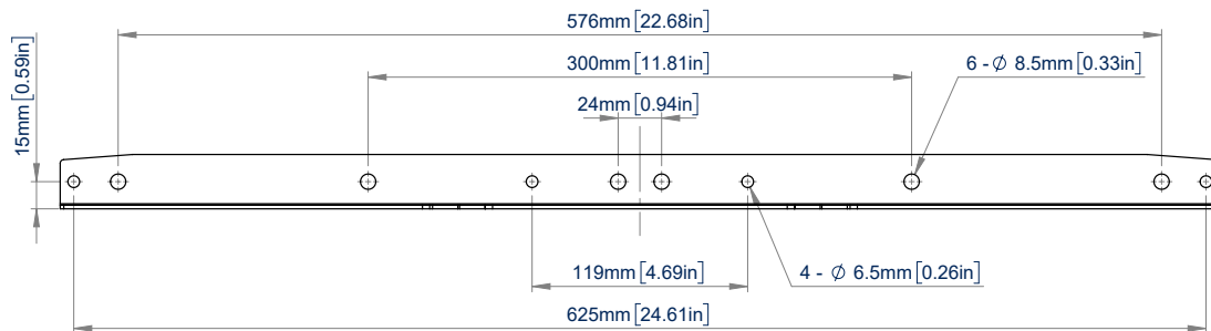
VISTA FRONTAL
