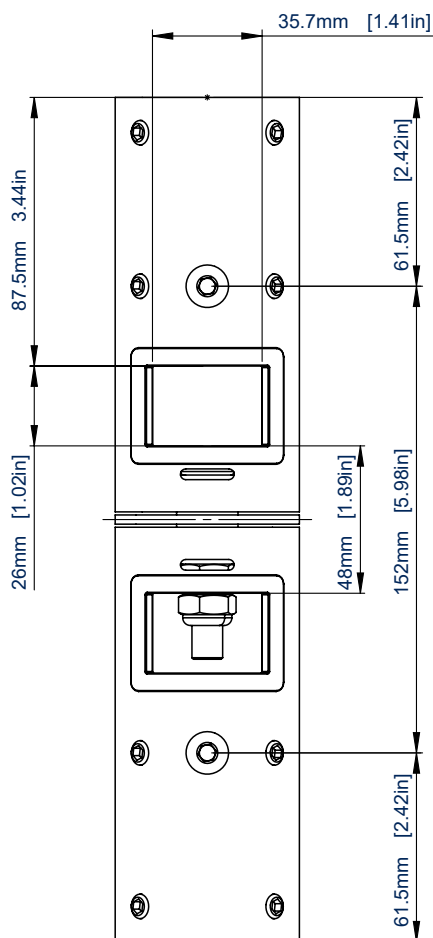
VISTA FRONTAL
