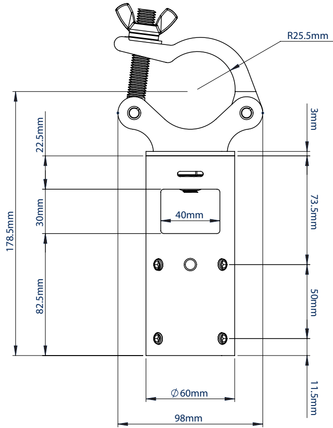
VISTA FRONTAL
