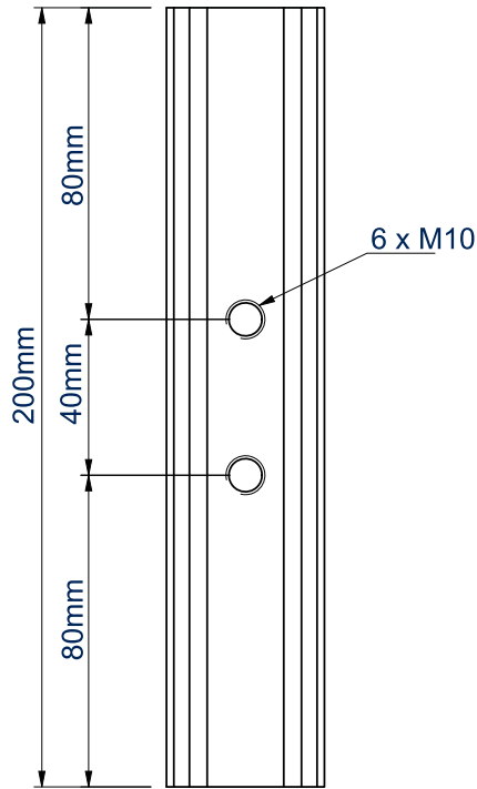
VISTA FRONTAL
