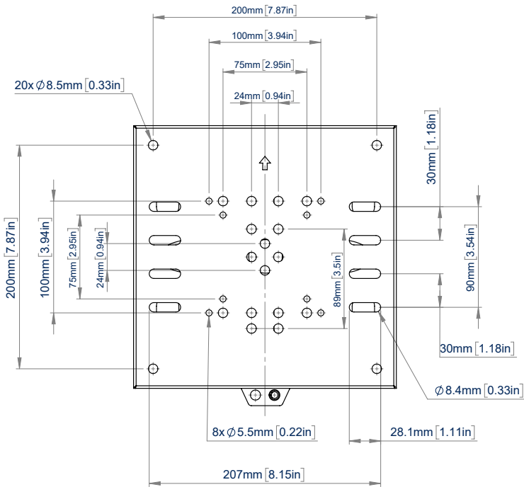
VISTA FRONTAL
