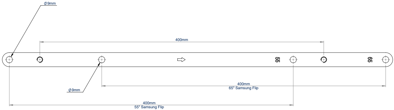
VISTA FRONTAL
