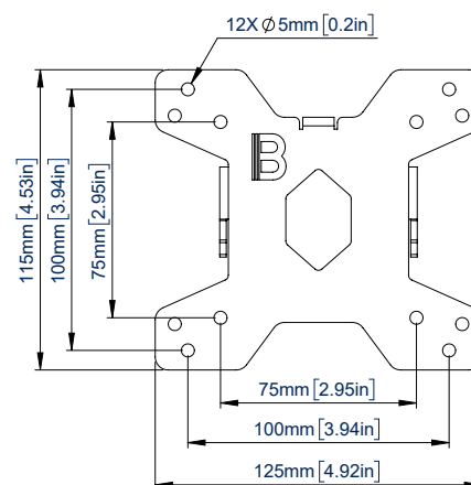
FRONT VIEW MOUNTING PLATE 100X100 OR 75X75
