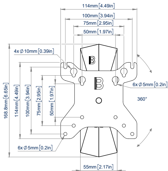
VISTA FRONTAL
