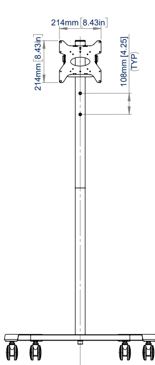
VISTA FRONTAL
