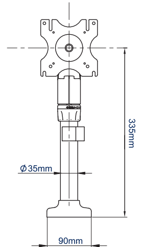
VISTA FRONTAL
