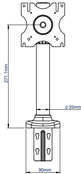
VISTA FRONTAL
