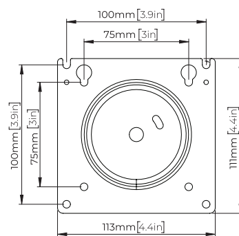
Wall Plate
