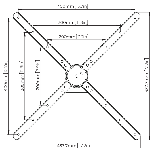
VESA Plate
