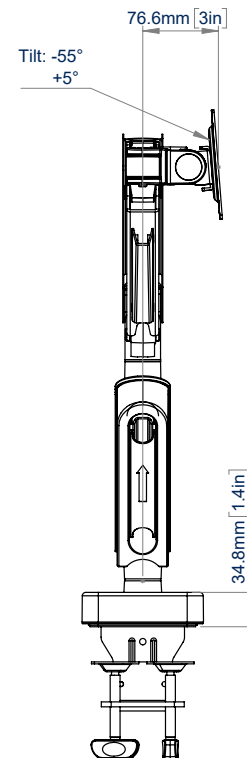
VISTA FRONTAL
