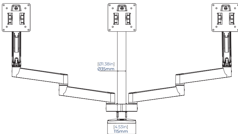
VISTA FRONTAL
