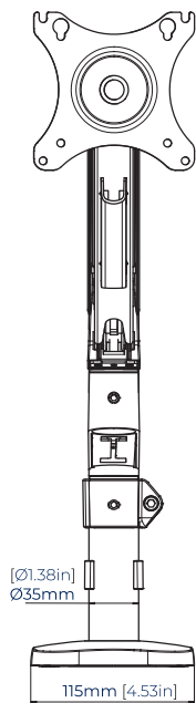
VISTA FRONTAL
