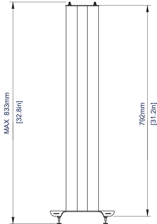
VISTA FRONTAL
