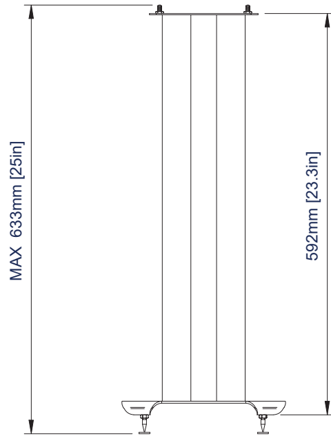
VISTA FRONTAL
