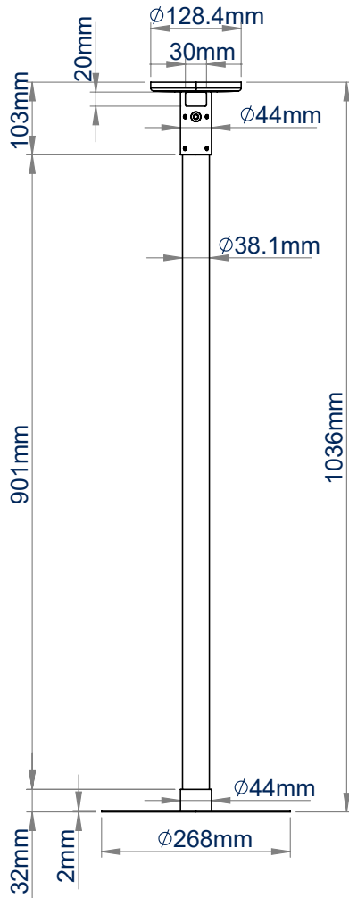
BT5961-FD100 VISTA FRONTAL
