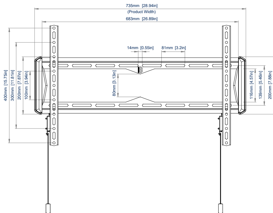
VISTA FRONTAL
