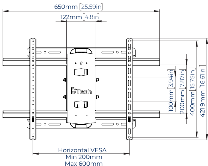
VISTA FRONTAL
