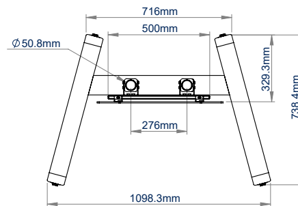
CHARIOT BASE
