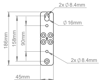
SUPPORT MURAL
