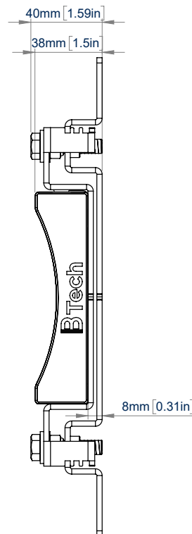
Side View with BT8390 Rail (Min Depth)
