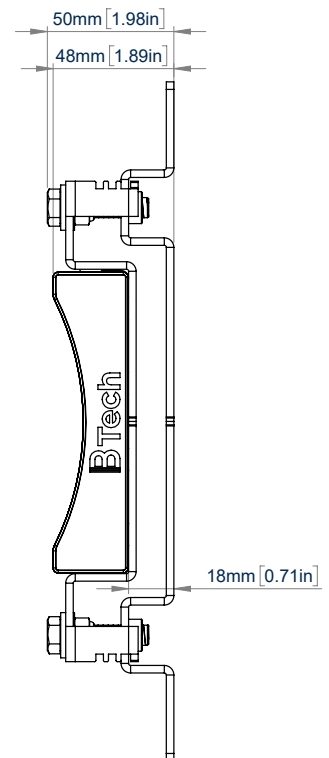
Side View with BT8390 Rail (Max Depth)
