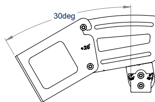
TILT 30 DEGREE
