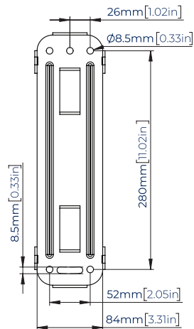
PLAQUE MURALE
