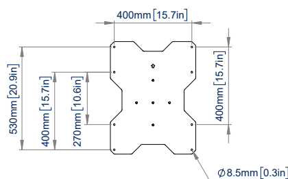
MOUNTING PLATE
