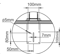
DETAIL B VC SHELF
