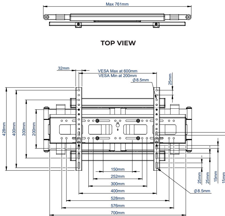
FRONT VIEW - CLOSED
