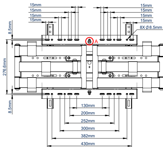
REAR VIEW - CLOSED
