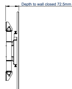
SIDE VIEW - CLOSED
