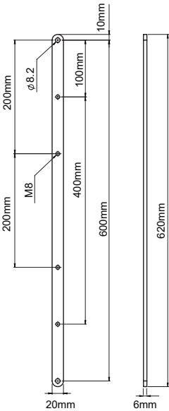
600mm Adaptor Arm
