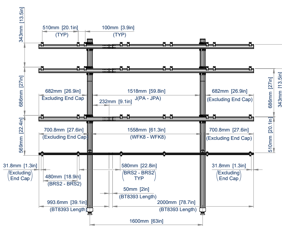
FRONT VIEW
