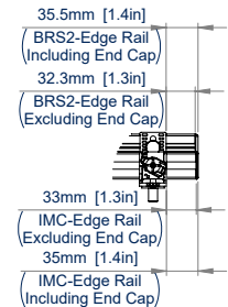
FRONT VIEW BT9240-BRS2
