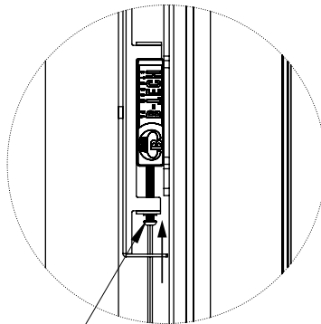
SAFETY SCREW
